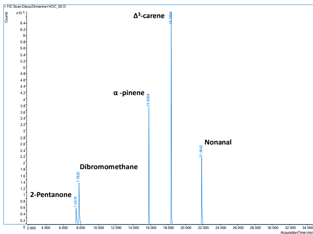
Figure 6 – Chromatogram of water sample from Disko Bay spiked with BVOCs standard
