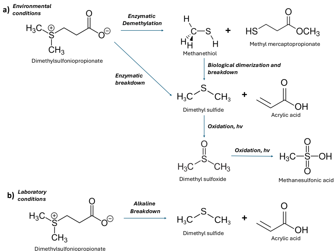
Figure 9 – Dimethylsulfoniopropionate breakdown reactions: a) in environmental conditions, b) in laboratory conditions
