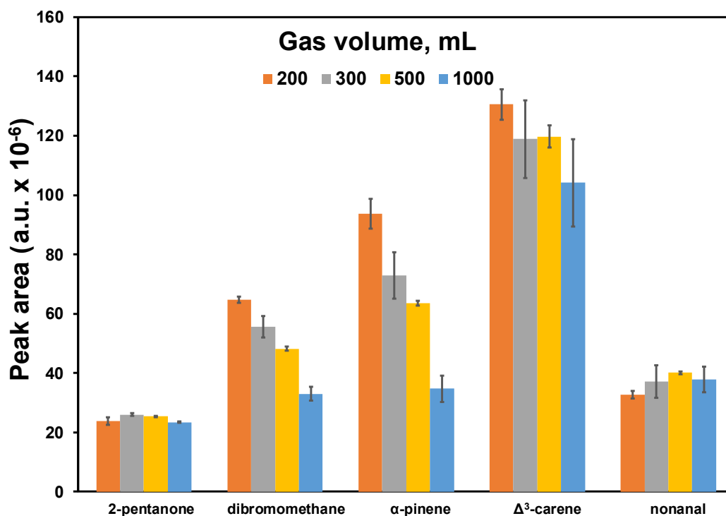
Figure 4 – Effect of drying gas volume on BVOCs responses. Trapping parameters: incubation temperature 30°C, sample temperature 30°C, gas volume 500 mL; Drying parameters: flow rate 100 mL min -1 , sorbent tube temperature 40°C
