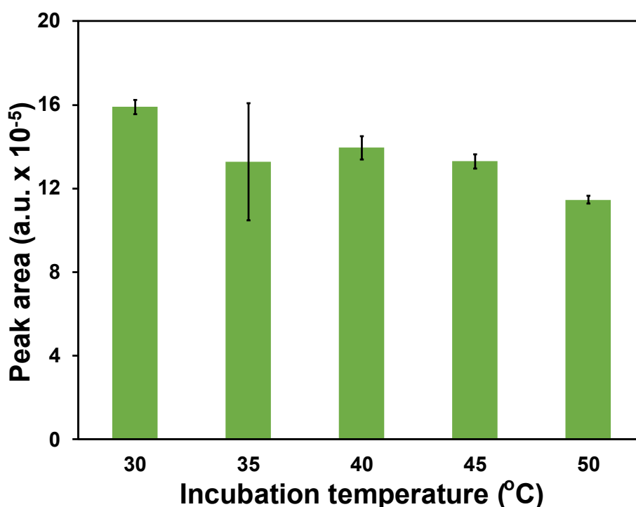
Figure 11 – The effect of vial incubation temperature on DMS response. Trapping parameters: sample temperature 30°C, gas volume 100 mL; Drying parameters: flow rate 100 mL min -1 , gas volume 500 mL, sorbent tube temperature 30°C
