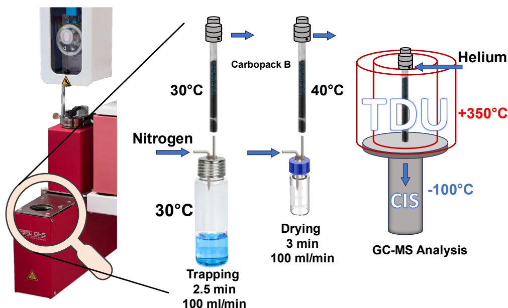
Figure 7 – Workflow of the dynamic headspace sampling process with sequential desorption in the TDU of the GC-MS system
