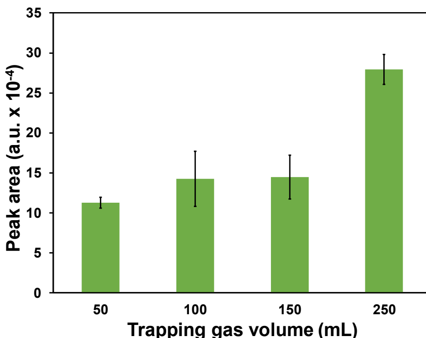
Figure 12 – The effect of trapping gas volume on DMS response. Trapping parameters: incubation temperature 30°C, sample temperature 30°C; Drying parameters: flow rate 100 mL min -1 , gas volume 500 mL, sorbent tube temperature 30°C
