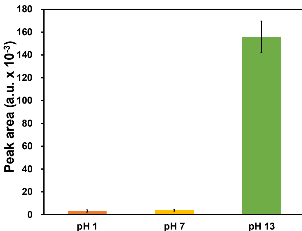
Figure 15 – The effect of pH on the preservation or derivatization of DMSP. DMSP concentration 1.26 \mu\text{g L}^{-1}
