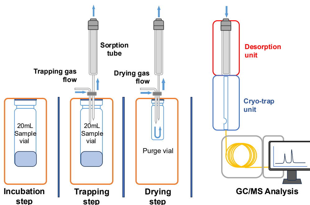
Figure 1 – Scheme of the dynamic headspace sampling process with sequential desorption to the TDU of the GC [54]
