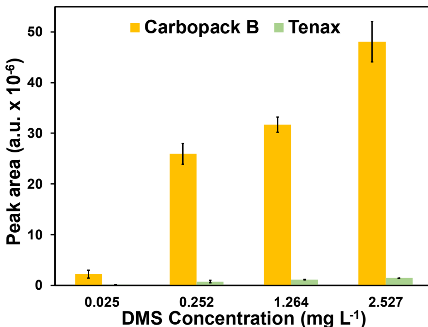
Figure 10 – The effect of sorbent types on DMS response. Trapping parameters: incubation temperature 30°C, sample temperature 30°C, gas volume 100 mL; Drying parameters: flow rate 100 mL min -1 , gas volume 500 mL, sorbent tube temperature 30°C
