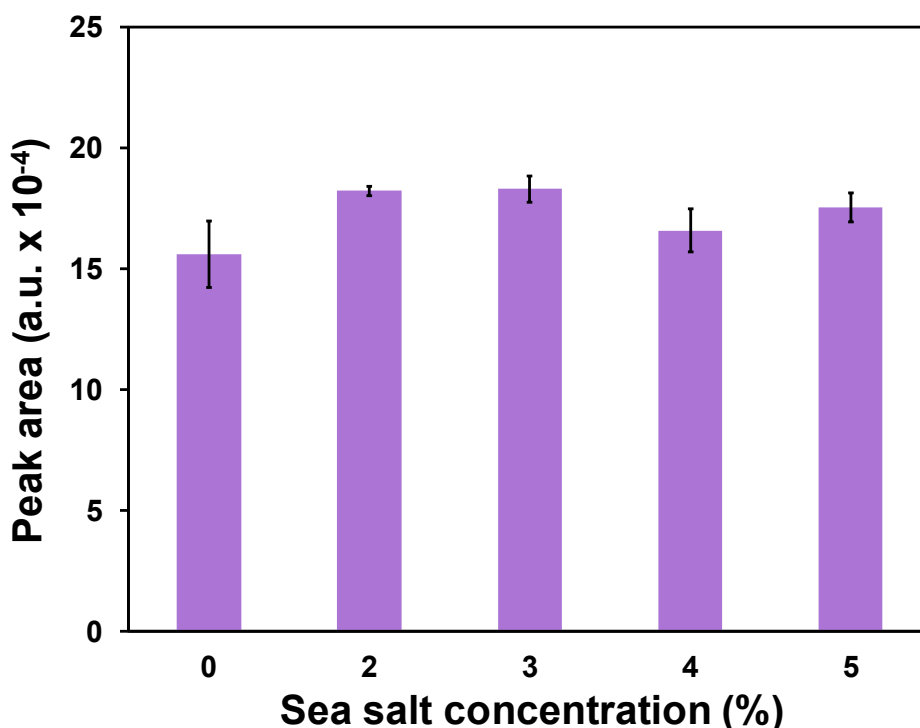
Figure 16 – Effect of sea salt concentrations on DMS response. DMSP concentration 1.26 \mu\text{g L}^{-1}
